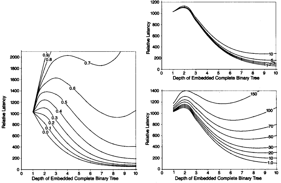
Fig. 18. At the left, the mean latency L as a function of n for various values of t with N = 1024 , k = 3 , and p = 0.3 . At the top right, the mean latency L as a function of n for various values of p with N = 1024 , k = 3 , and t = 1.0 . At the bottom right, the mean latency L as a function of n for various values of k with N = 1024 , p = 0.3 , and t = 1.0 .
