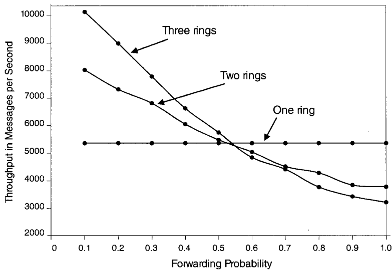
Fig. 16. Throughput for the three topologies as a function of forwarding probability.
